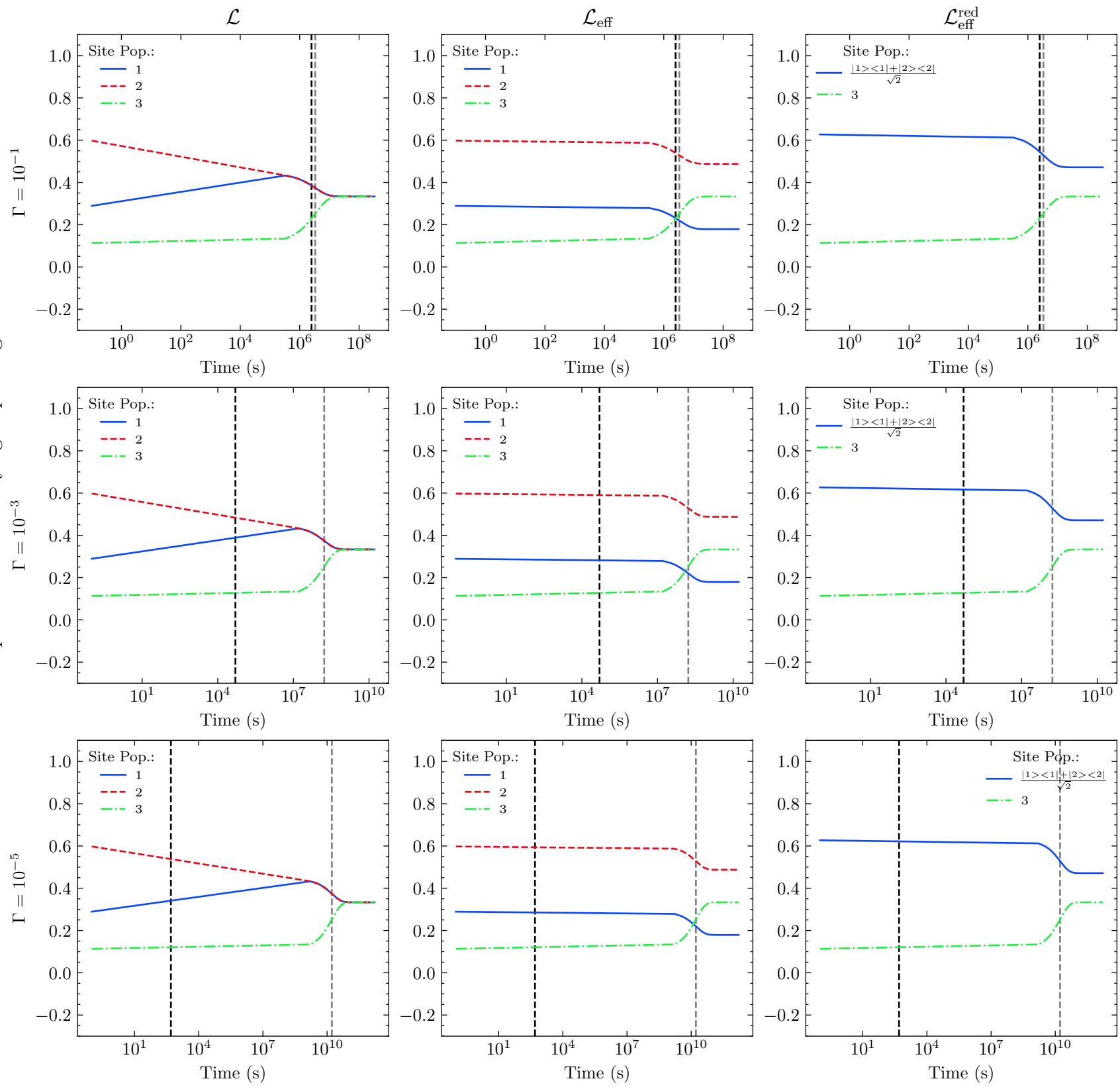
Time Evolution of Site Populations under \mathcal{L} , \mathcal{L}_{\text{eff}} , and \mathcal{L}_{\text{eff}}^{\text{red}} N=3 ; J = 10^{-1} ; \epsilon = 10^{-4}
